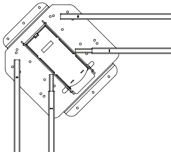
Universal Corner Bracket
